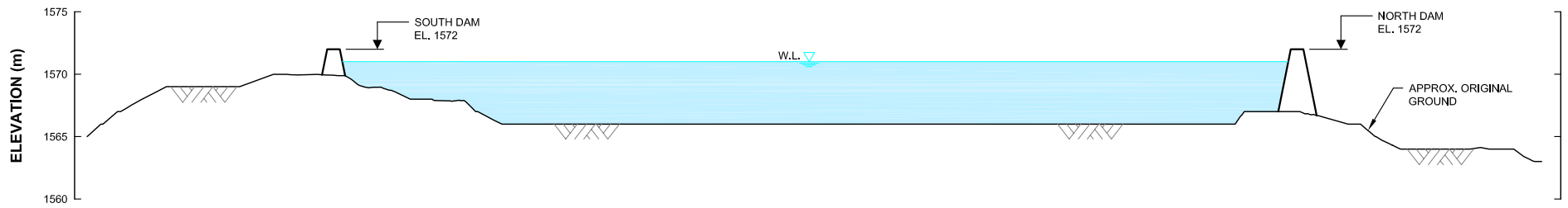
TYPICAL SECTION HORIZ. SCALE A VERT. SCALE B
