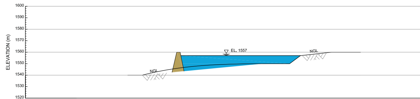
3 SECTION 7.1-1 HORIZONTAL: SCALE A VERTICAL: SCALE B
