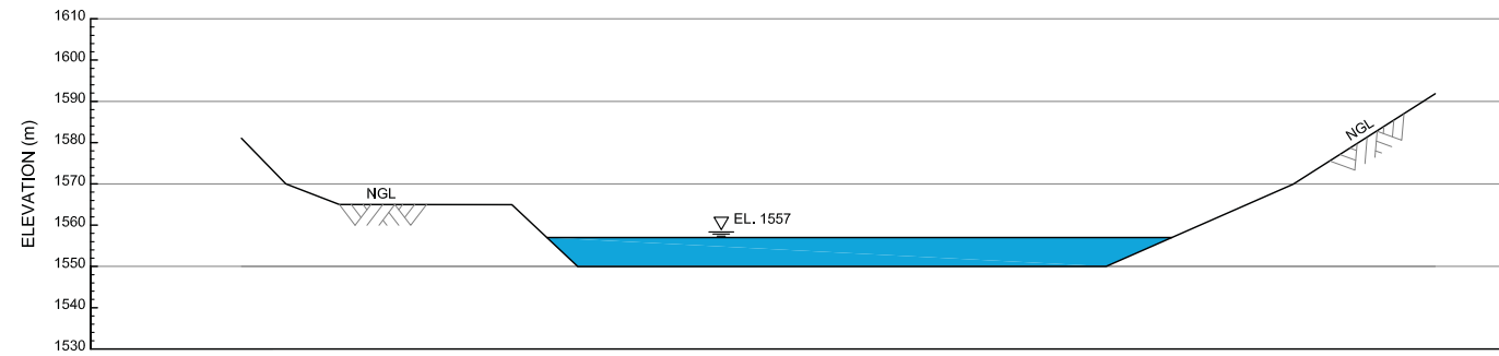
1 SECTION 7.1-1 HORIZONTAL: SCALE A VERTICAL: SCALE B
